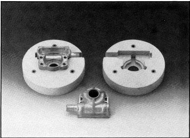
Reusable nest to hold gearbox securely (precise negative shape) and eliminate scratching of part during robotic assembly process.
