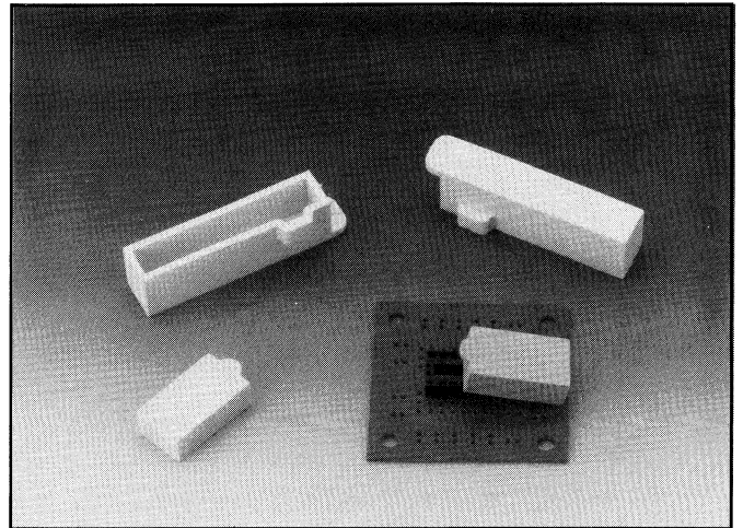
Reusable covers for printed circuit board components used during wave soldering and conformal coating process. (eliminate costly masking).
